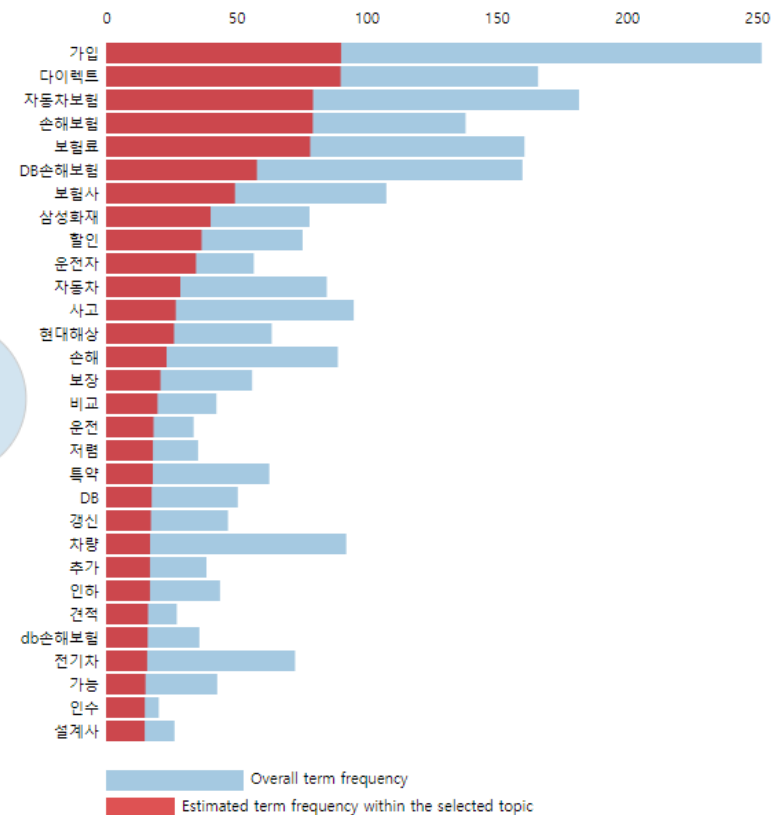
Top-30 Most Relevant Terms for Topic 2 (33.6% of tokens)
